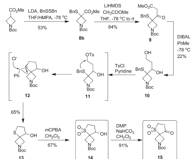
Scheme 2. Synthesis of Spirocyclic Modules 14 and 15
