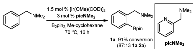
Scheme 1. Control Experiment Using Dimethylpicolylamine
