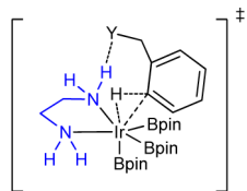
Figure 1. Proposed bifunctional directing effect.
