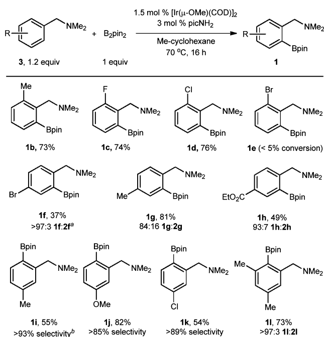
Figure 3. Scope of amine directing group.
