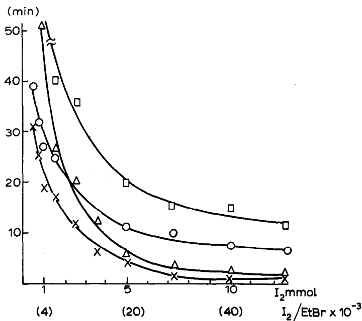
Fig. 1. Initiation time vs. I_2/EtBr at 36^\circ C . \Delta , initiation time with heating and stirring; \square , completion time with heating and stirring; \times , initiation time with ultrasonic irradiation; \circ , completion time with ultrasonic irradiation.
