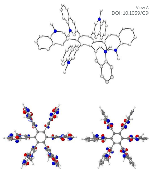
Figure 3. Most stable conformation of 25 (calculated) (above). HOMO (left) and LUMO (right) of 25 (3,3)-1,3,5.
