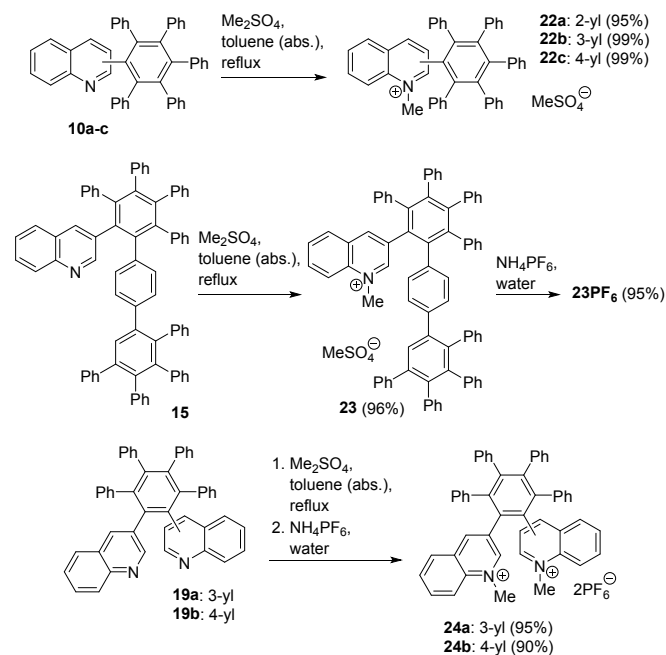
Scheme 7. Methylation of quinoline-based HABs.
