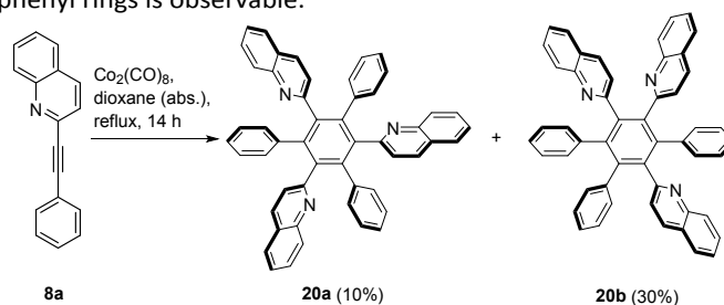
Scheme 5. Cobalt-catalyzed [2+2+2]-cyclotrimerization.
