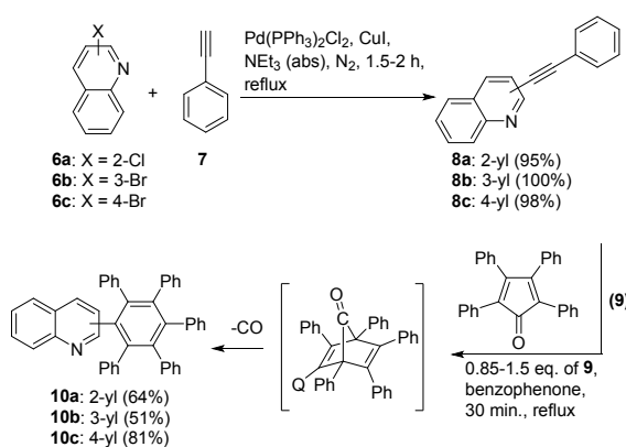
Scheme 2. Synthesis of monoquinoline-substituted HHABs.
