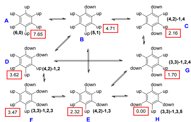
Figure 2. Eight energy-minimized rotamers of 25 , showing which can be directly interconverted by rotation of a single substituent. Relative energies (in \text{kJ mol}^{-1} ) are shown in red boxes.
