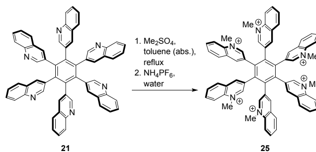
Scheme 8. Methylation of perquinoline-substituted HAB 21 .
