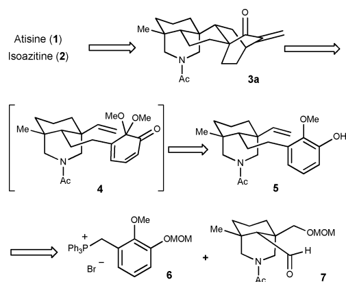
Scheme 1 Retrosynthetic analysis for (±)-atisine and (±)-isoazatine.
