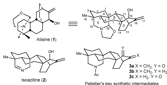
Fig. 1 Structures of atisine, isoazitine, and Pelletier's key synthetic intermediates.
