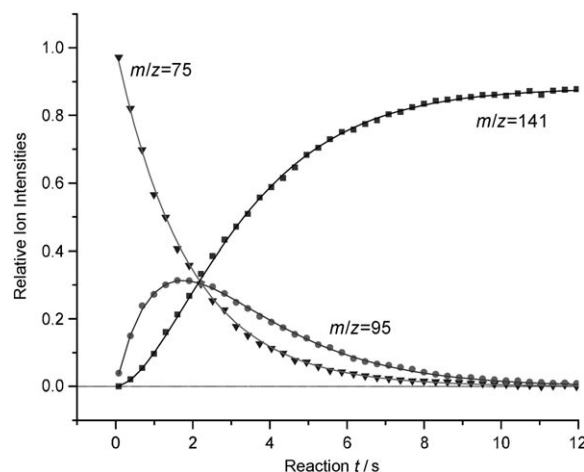
Figure 1. Temporal evolution of the relevant ion intensities. B_{\text{ref}} = HCO_2Et . P_I = 3.3 \times 10^{-8} mbar (nominal pressure).
