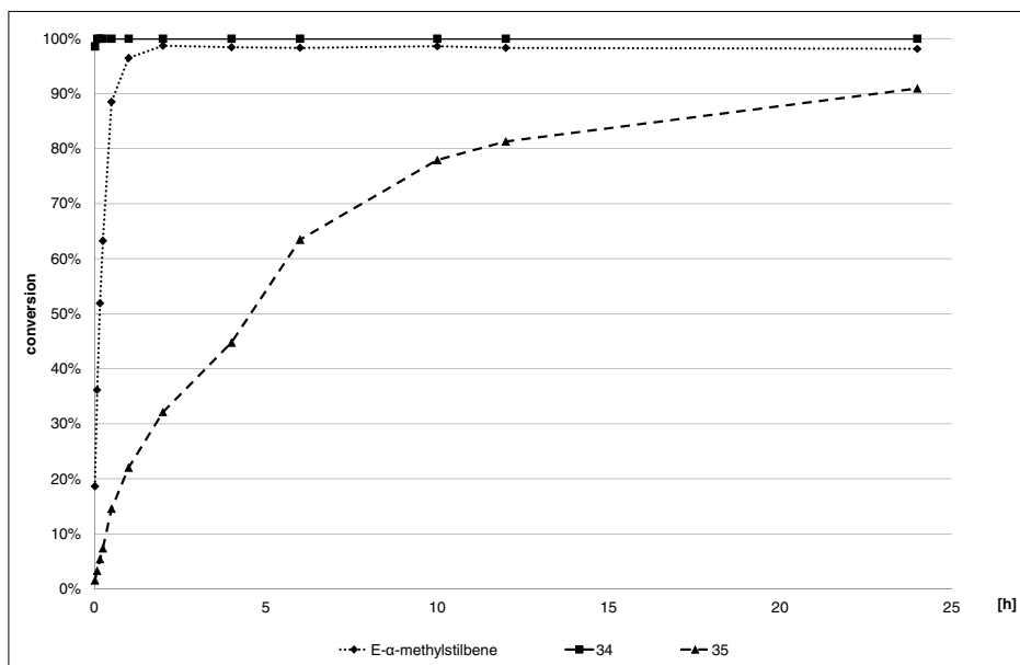
Fig. 4. Conversion over time for the hydrogenation of \alpha,\beta -unsaturated boronic esters 34 , 35 and E -methylstilbene.
