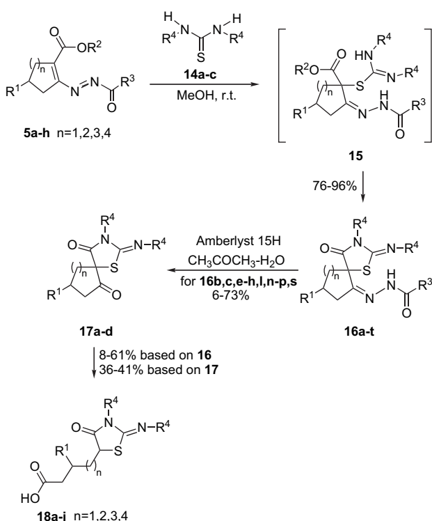
Scheme 4.
