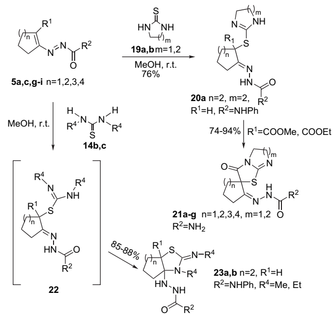
Scheme 5.
