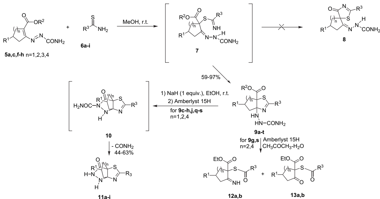
Scheme 3.
