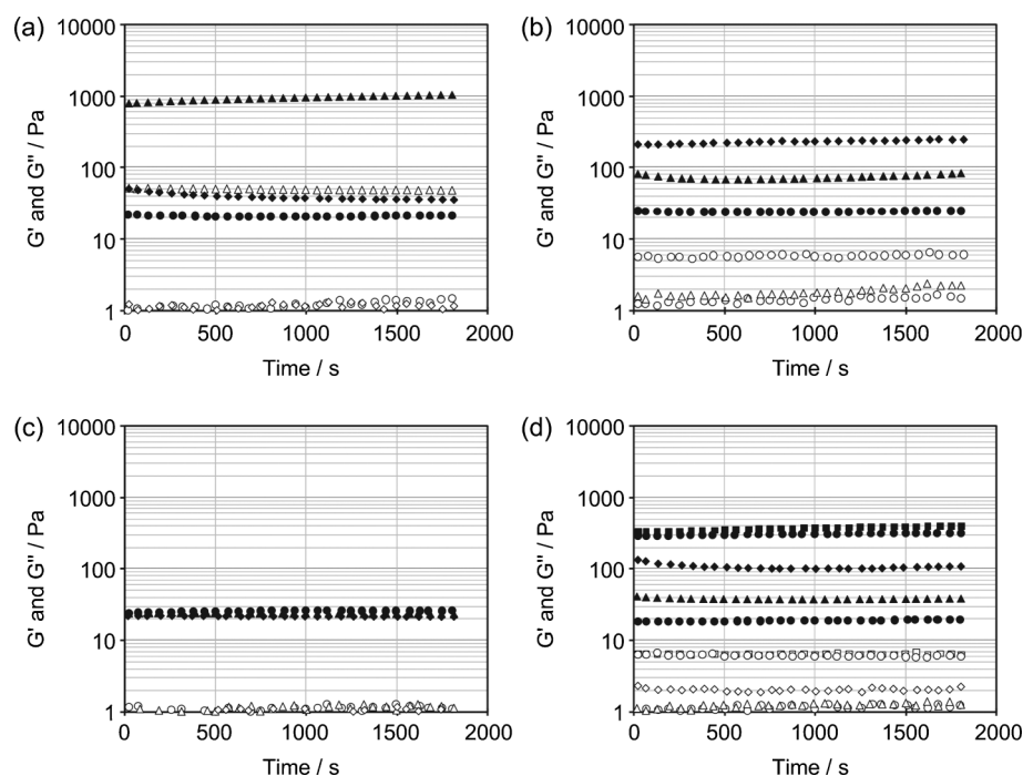
Fig. 7 Increase of G' (full symbols) and G'' (empty symbols) for hydrogels of 2 (a) and 2 in the presence of 0.5 eq. of ( R )-citronellal ( 14 , b), Triplal ® ( 13 , c), or an equimolar mixture of 13 and 14 (0.25 eq. each, d) after several consecutive cooling and heating cycles.
