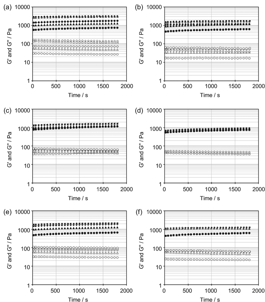
Fig. 6 Increase of G' (full symbols) and G'' (empty symbols) for hydrogels of 1 (a) and 1 in the presence of 0.5 eq. of 24 (b), menthone ( 19 , c), ( R )-citronellal ( 14 , d), Triplal® ( 13 , e) or an equimolar mixture of 13 and 14 (0.25 eq. each, f) after several consecutive cooling and heating cycles.
