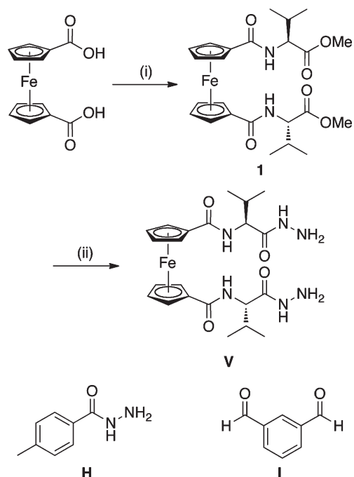
Figure 2. Building blocks \text{Fc}-[\text{CO}-\text{Val}-\text{NHNH}_2]_2 ( V ), isophthalaldehyde ( I ), and 4-methylbenzhydrazide ( H ). Reagents and conditions for the synthesis of V : (i) \text{H}-\text{Val}-\text{OMe} , \text{HOBt} , \text{EDC} , \text{Et}_3\text{N} , \text{DMF} , overnight, 72%; (ii) \text{N}_2\text{H}_2 \cdot \text{H}_2\text{O} , \text{MeOH} , 2 days, 77%.
