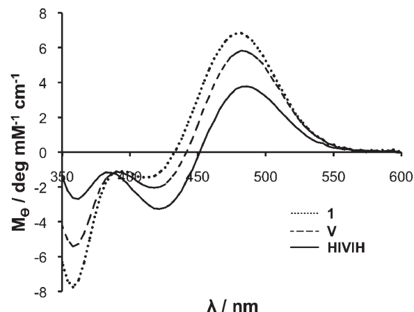
Figure 6. CD spectra of \text{Fc}[\text{CO-Val-OMe}]_2 ( 1 ), V , and HIVIH (2 mM in 96:4 \text{CHCl}_3/\text{MeOH} ).
