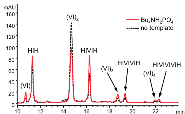
Figure 3. HPLC chromatogram (290 nm) showing the equilibrium distribution of components in a DCL formed from V (0.5 mM), I (0.5 mM), and H (1 mM) in 96:4 \text{CHCl}_3/\text{MeOH} solution containing 1-naphthoic acid (20 mM) in the absence (dashed black curve) and presence (solid red curve) of \text{Bu}_4\text{NH}_2\text{PO}_4 (0.25 mM).
