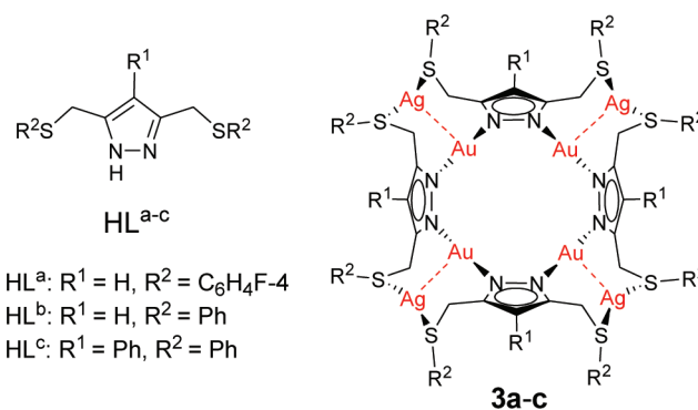
Figure 2. Pyrazolate ligands \text{HL}^{\text{a-c}} with appended thioether substituents and the new multinuclear coinage metal complexes 3a–c .
