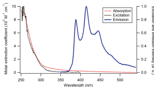
Figure 6. Photoluminescence spectra of 3b . The emission spectrum (blue) was detected after excitation at 280 nm, while the excitation spectrum (dashed black) monitored the emission at 415 nm. The red line is the absorption spectrum of 3b in 2-methyl-THF at room temperature.
