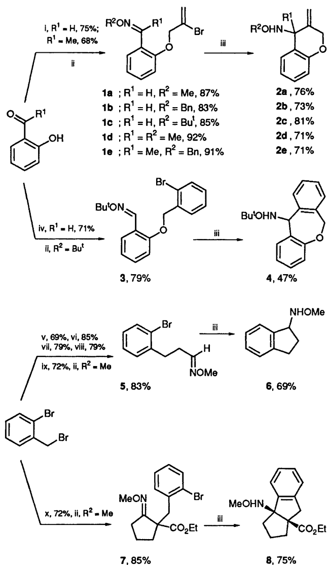
Scheme 1 Reagents and conditions: i, BrCH_2C(Br)=CH_2 , K_2CO_3 , Me_2CO , reflux 5 h; ii, R^2ONH_2 \cdot HCl , pyridine, room temp., 4 h; iii, Bu_3SnH , AIBN, PhH , reflux; iv, 2- BrC_6H_4CH_2Br , K_2CO_3 , Me_2CO , reflux 5 h; v, NaOEt , EtOH , CH_2(CO_2Et)_2 , reflux 12 h; vi, NaOH , heat, then HCl , heat; vii, EtOH , cat. H_2SO_4 , reflux; viii, LiAlH_4 , Et_2O , reflux, 2 h; ix, (COCl)_2 , Me_2SO , Et_3N ; x, NaH , tetrahydrofuran, 1,3-dimethyl-3,4,5,6-tetrahydro-2(1 H )-pyrimidinone, ethyl 2-oxocyclopentane carboxylate, reflux
