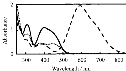
Figure 2. UV-vis spectra of trans - 4 in MeCN at 23.3 °C (solid line), after photoirradiation at 405 nm (dotted line), and after addition of 7.5 equivalents of \text{CF}_3\text{SO}_3\text{H} (dashed line).
