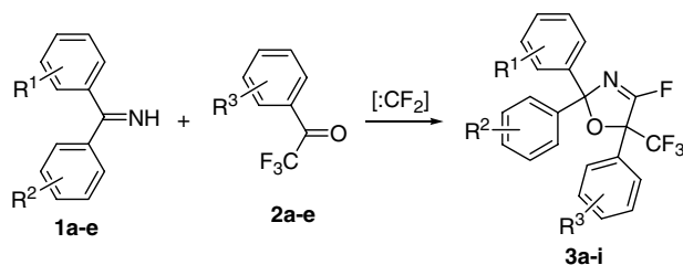
Scheme 2. The synthesis of fluorooxazolines 3a–i .
