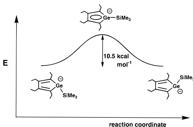
Figure 7. Reaction coordinate diagram for inversion in the complex [Li(12\text{-crown-}4)][C_4Et_4GeSiMe_3] ( 40 ).
