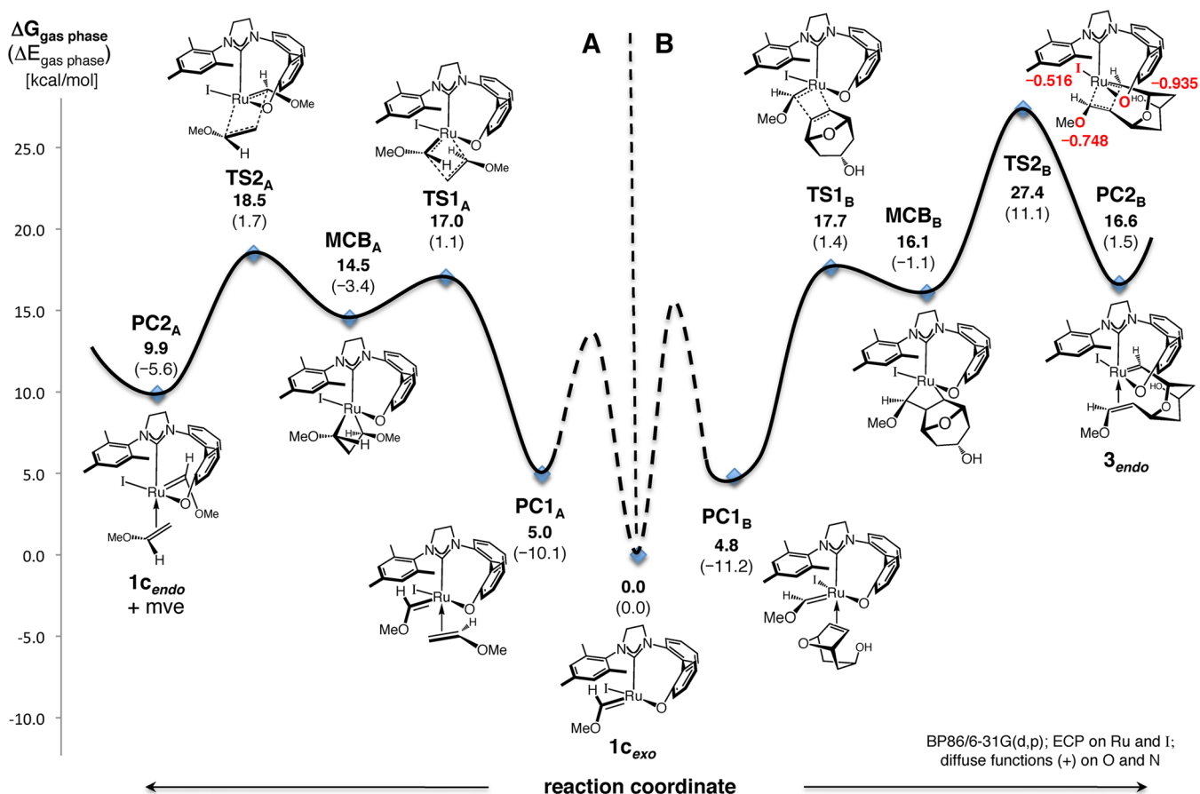
Figure 1. Computed energy barriers ( \Delta G in kcal/mol; bold values) for nonproductive olefin metathesis reactions of methylvinyl ether (A, 1c_{exo} \rightarrow 1c_{endo} + mve ) and productive ring-opening/cross-metathesis (ROCM) of the exo carbene derived from the same enol ether with oxabicyclic alkene 2 (B, 1c_{exo} \rightarrow 3_{endo} ; non-Curtin–Hammett pathway). \Delta E values (gas phase) are provided in parentheses. mve = methyl vinyl ether; PC = \pi complex, TS = transition state; MCB = metallacyclobutane.
