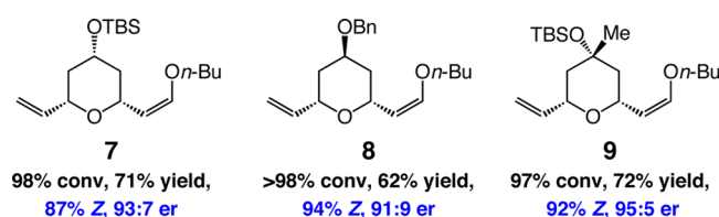
Scheme 3. Enantioselective Ru-Catalyzed ROCM with Various Oxabicycles
