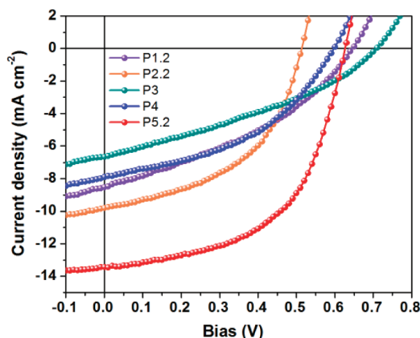
Figure 9. I – V curves of P1.2 , P2.2 , P3 , P4 , and P5.2 based PSCs (at best polymer:PCBM composition) under AM 1.5 solar illumination, 100 \text{ mW cm}^{-2} . Devices with postpolymer processing thermal treatment at 70^\circ\text{C} (30 min). The device structure is ITO/PEDOT/PX:PC 71 BM/LiF/Al with PX = P1.2 , P2.2 , P3 , P4 , or P5.2 .
