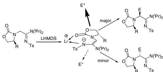
Fig. 1. Proposed transition state of the asymmetric \alpha -alkylation.
