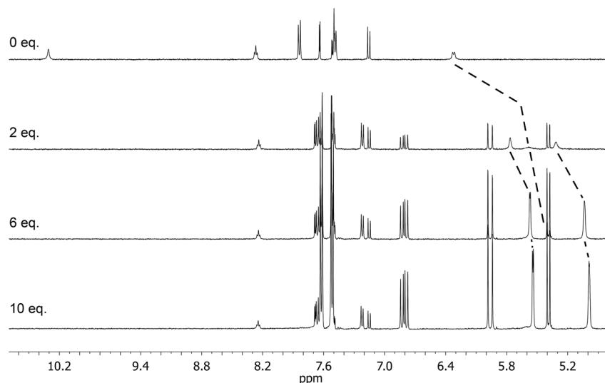
Fig. 3 Overlay of characteristic ^1\text{H} NMR spectra (DMSO- \text{d}_6 ) obtained during the titration of GLIB vs. VBTA, showing the disappearance of the acidic sulfonylurea proton and the movement of the second sulfonylurea proton, as well as the movement of the methacrylate vinyl protons. From top to bottom, 0 eq., 2 eq., 6 eq. and 10 eq. of VBTA added to GLIB.
