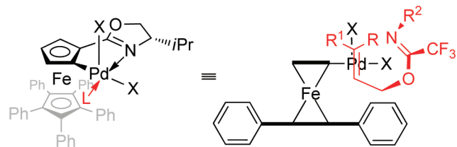
Figure 13. Working hypothesis to rationalize the stereospecific reaction outcome for the rearrangement of allylic trifluoroacetimidates. Face-selective olefin coordination followed by outer-sphere attack of the imidate N-atom at the olefin can explain why the configuration of the new stereocenter switches for different geometric isomers and why quaternary stereocenters can be generated with high stereocontrol.
