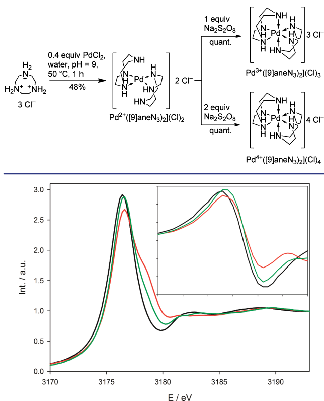
Figure 3. Pd L_3 -edge XANES spectra of the [\text{Pd}^{x+}([\text{9}]\text{aneN}_3)_2](\text{Cl})_x reference system: x = 2 (black line), 3 (red line), and 4 (green line) are compared. The first derivatives of the edge region are shown as inset.
