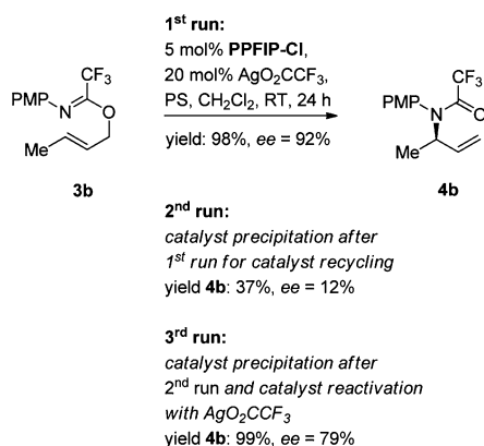
Scheme 6. Study of the Catalyst Deactivation and Reactivation (PS = Proton Sponge = 1,8-Bis(dimethylamino)naphthalene)
