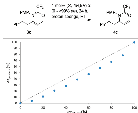
Figure 12. Negative nonlinear effect for the allylic imidate rearrangement of 3c using ( Sp ,4 R ,5 R )- 2 with catalyst ee values ranging from 0 - >99%. With almost enantiopure catalyst product 4c is formed with 99.6% ee. The NLE suggests the existence of higher catalyst aggregates, most likely dimers, in equilibrium with the monomeric complex binding the substrate.
