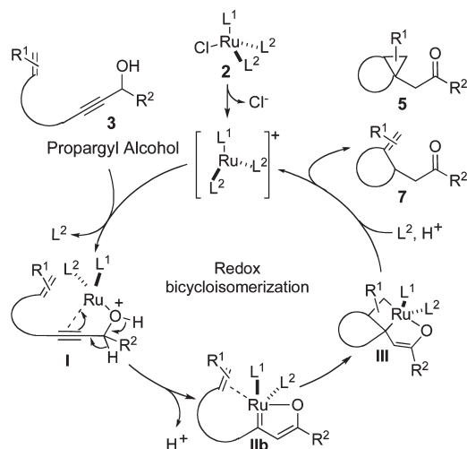
Scheme 3. Proposed Catalytic Cycle
