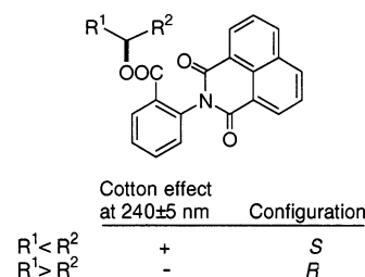
Figure 1. Correlation between the size of R^1, R^2 (absolute configuration) and the sign of the NAB Cotton effect.
