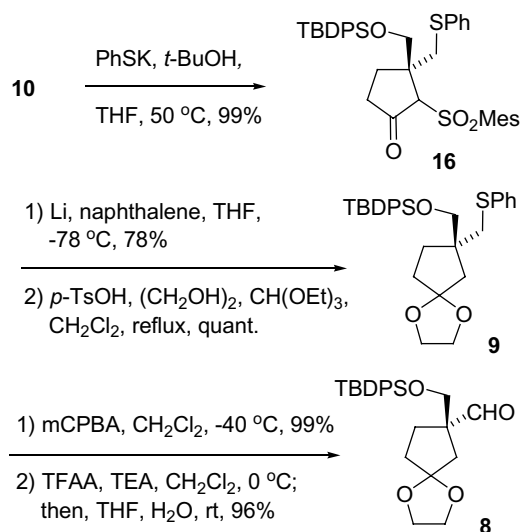
Scheme 4. Enantioselective synthesis of 8 .
