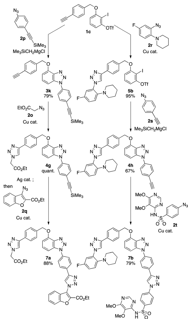
Scheme 3 Synthesis of tris-triazoles by three sequential cycloadditions. See ESI† for details of the conditions.
