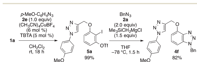
Scheme 2 Bistriazole synthesis by sequential azide–alkyne/azide–aryne cycloadditions.
