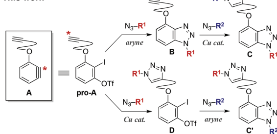
Scheme 1 Synthesis of unsymmetrical bistriazoles by sequential azide–alkyne cycloadditions.
