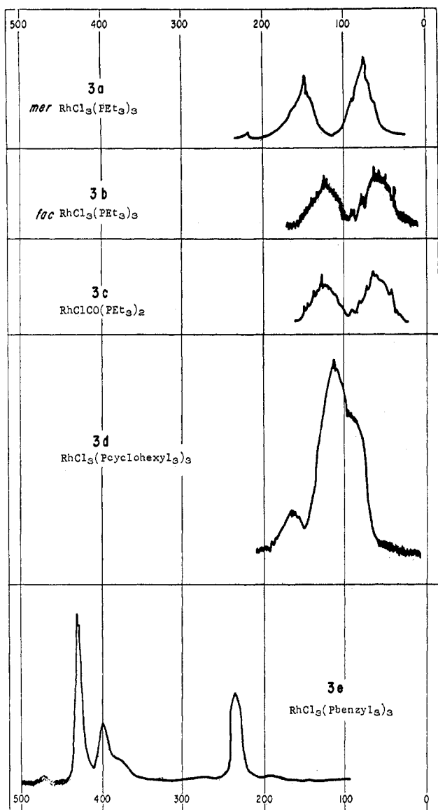
Figure 3.—Nmr spectra of trialkylphosphine complexes.
