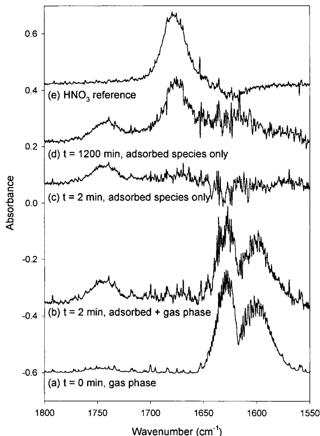
Figure 2. FTIR spectra of 2.9 Torr of \text{NO}_2 in \text{N}_2 (total pressure 508 Torr) (a) gas-phase only, (b) gas-phase plus surface-adsorbed species, (c) subtracted spectrum (b – a) showing the spectrum due to the adsorbed species, and (d) same as (c) but 20 h later; (e) reference spectrum of \text{HNO}_3 adsorbed on porous glass; 0.57 Torr of \text{HNO}_3 was added to the cell for 5 min and then pumped away before recording the spectrum. The porous glass had been heated under vacuum before the exposure to \text{NO}_2 . All spectra are on the same scale.
