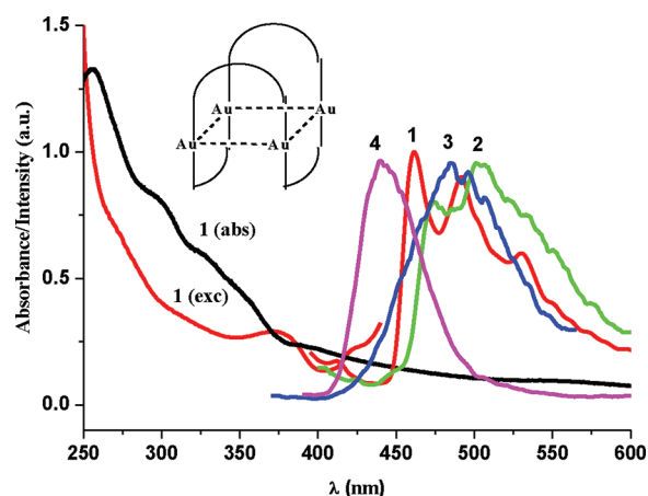
Figure 2. Absorption spectrum of 1 solution in 5 \times 10^{-5} M CH 2 Cl 2 (black), excitation (red), and emission spectra (red) in the solid state at 77 K. Emission spectra for 2 (green), 3 (blue), and 4 (magenta) in solid state at 77 K.
