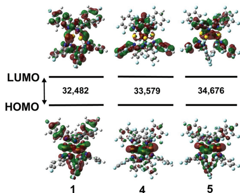
Figure 3. Frontier orbitals (HOMO and LUMO) for model systems [\text{Au}(\text{ArN})_2\text{C}(\text{H})]_4 (Ar = 4- \text{FC}_6\text{H}_4 , 1; 2,3,5,6- \text{F}_4\text{C}_6\text{H} , 4; and \text{C}_6\text{F}_5 , 5). The HOMO–LUMO gaps are in \text{cm}^{-1} H atoms removed.
