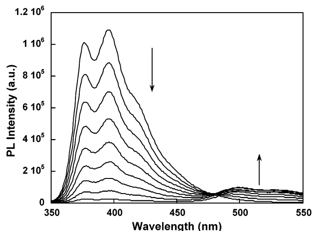
Figure 1. Emission spectra for mixtures of C 8 with 3 in water. [\mathbf{C}_8] = 2.0 \times 10^{-6} M, [\mathbf{3}] = 3.0 \times 10^{-8} M to 1.0 \times 10^{-6} M.
