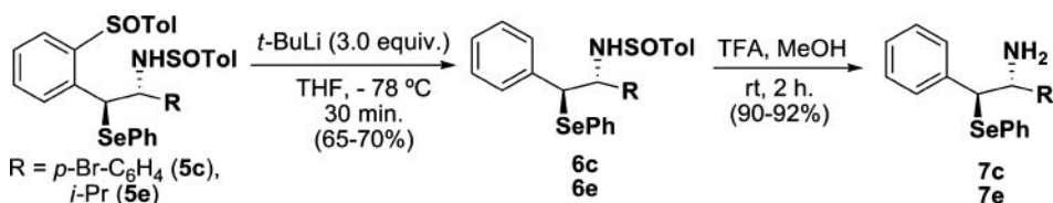
Scheme 6
