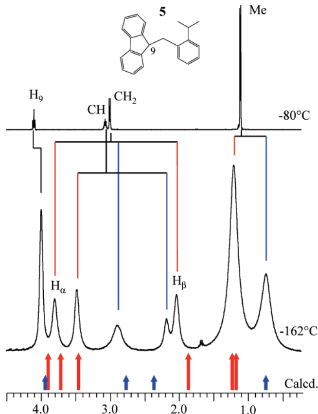
FIGURE 8. 1 H NMR spectrum (600 MHz in CHF 2 Cl/CH 2 Cl 2 ) of the aliphatic region of 5 at two different temperatures. The arrows (red for the major and blue for the minor conformer) represent the DFT calculated shifts (all moved upfield by 0.34 ppm).
