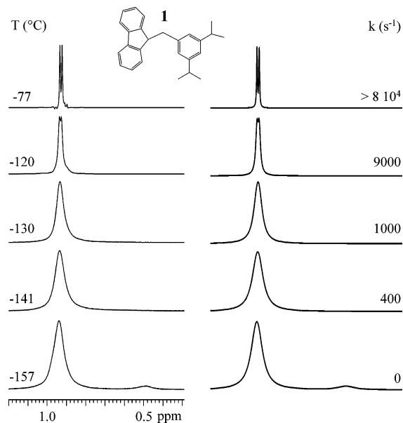
FIGURE 1. Temperature dependence of the methyl signal (600 MHz in \text{CHF}_2\text{Cl}/\text{CH}_2\text{Cl}_2 ) of compound 1 (left). On the right the spectral simulation with the rate constants indicated.
