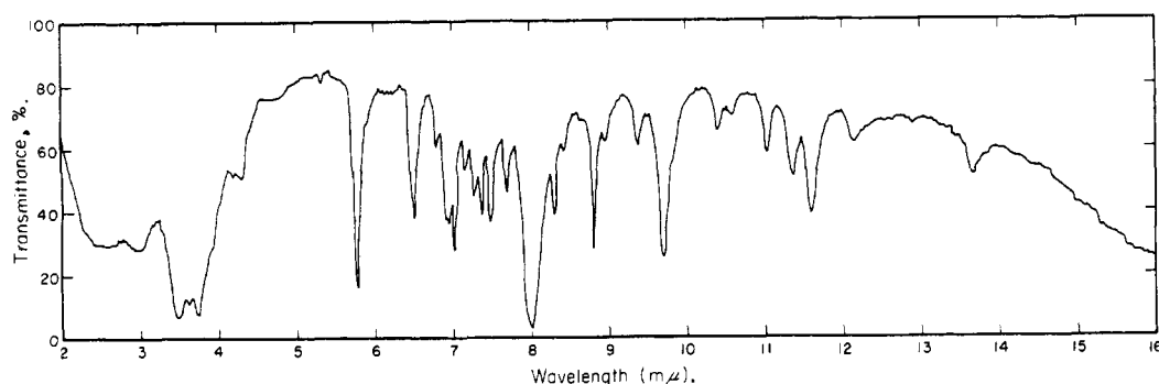
Fig. 1.—Infrared spectra of synthetic ethyl thiazolidine-4-carboxylate hydrochloride (VII).
