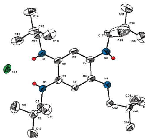
Figure 3. View of the crystal structure of 5·HCl .
