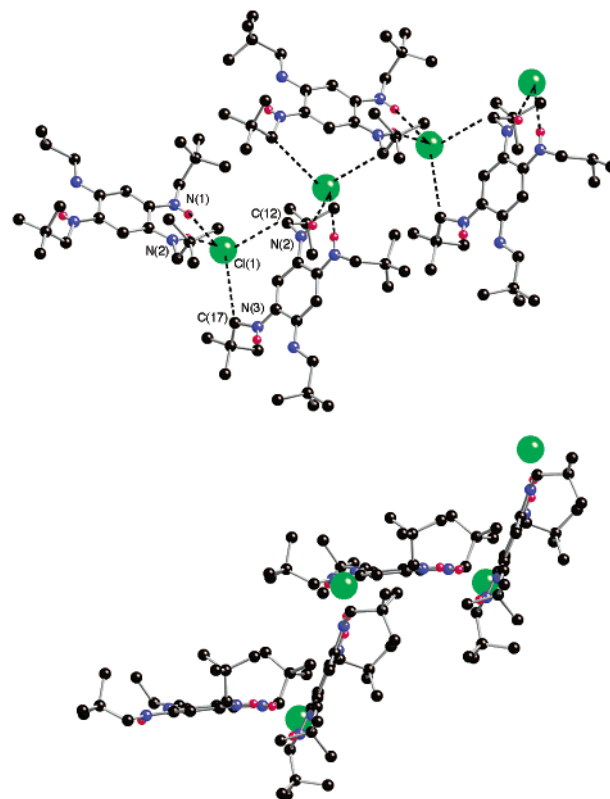
Figure 6. Crystallmaker top and side views of the cation–anion associations in 5 ·HCl. Color coding: nitrogen, blue; hydrogen, red; chloride, green.
