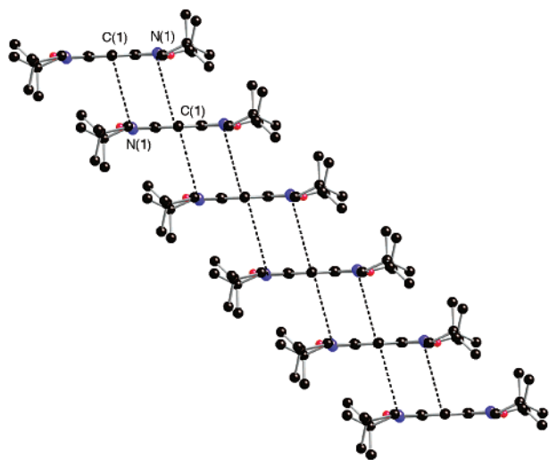
Figure 5. Crystallmaker side view of the stacking of 5 in the solid state. Color coding: nitrogen, blue; hydrogen, red.
