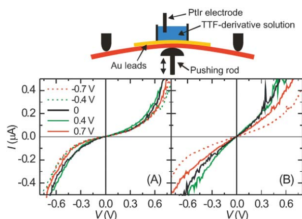
Fig. 3 I – V characteristics, at different gate voltages, for a wide open (A) and almost closed (B) break junction immersed in a solution of 4 . The inset shows a schematic of the break junction setup working in liquid.
