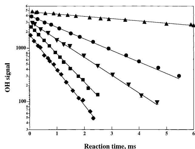
Figure 2. Plots of ln[OH] t vs time at 298 K for different ClO under conditions of excess O 3 . Values of k 1 ' were obtained from the slope of such plots at various ClO concentrations.
