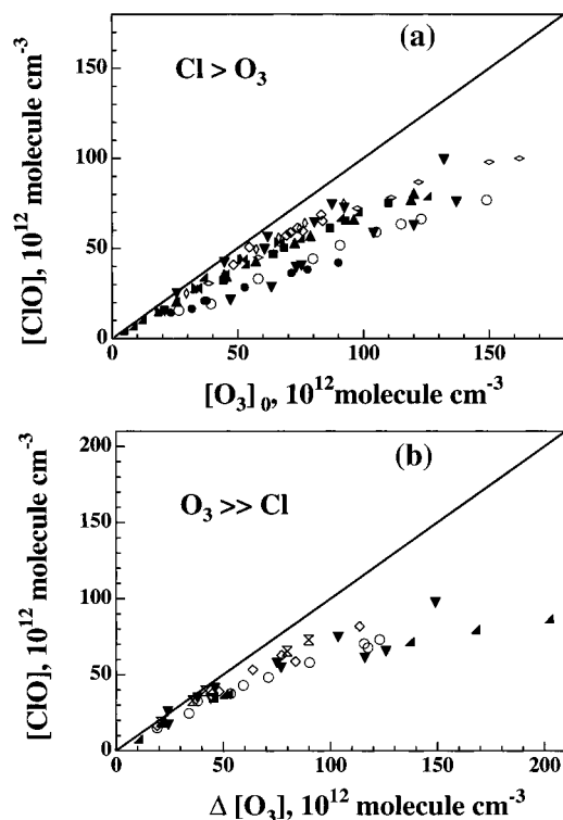
Figure 6. (a) Plot of the measure [ClO] vs [O_3]_0 obtained under conditions where O_3 was depleted during ClO production. (b) Plot of [ClO] vs \Delta[O_3] for a few experiments done with O_3 in excess. Each of the symbols represents data taken during different days or under varying experimental conditions. If the production of ClO from O_3 were stoichiometric, the data points would fall on the 1-to-1 lines shown.
