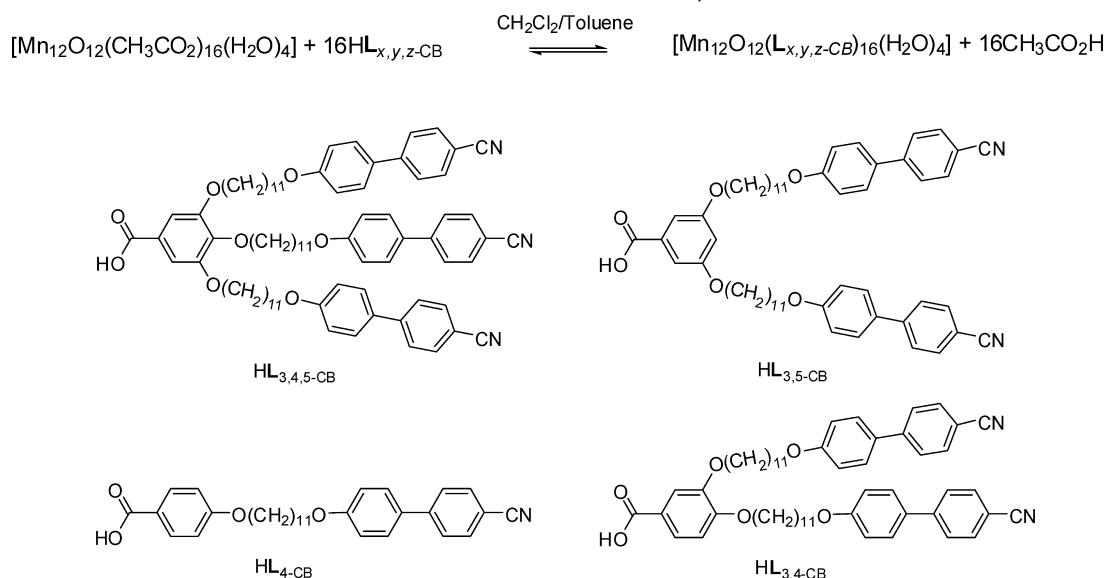
Scheme 1. Schematic Representation of the Solvent-Mediated Ligand-Exchange Reaction and Chemical Structures of the Cyanobiphenyl-Substituted Benzoic Acid Derivatives Used as Ligands ( \text{HL}_{x,y,z}\text{-CB} )
