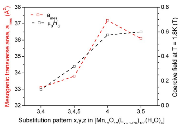
Figure 10. Evolution of the transverse molecular area, a_{\text{mes}} , and coercive field, \mu_0 H_C , as a function of the ligand-substitution patterns.
