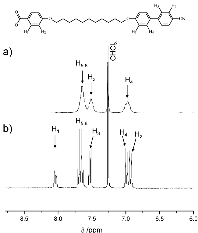
Figure 2. ^1\text{H} NMR spectra with numbering scheme for [\text{Mn}_{12}\text{O}_{12}(\text{L}_{3,4,5}\text{-CB})_{16}(\text{H}_2\text{O})_4] (top) and \text{HL}_{4\text{-CB}} (bottom) in \text{CDCl}_3 at 298 K.
