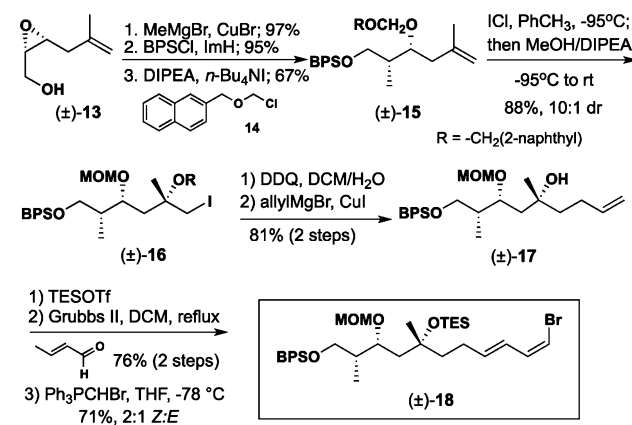
Scheme 2. Application to the C9–C19 Fragment Synthesis
