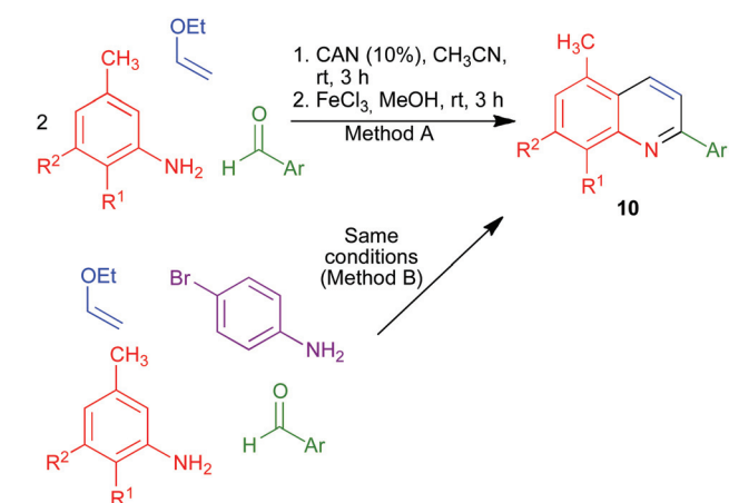
Scheme 6 Synthesis of 2-arylquinolines from anilines, aromatic aldehydes and vinyl ethers.
