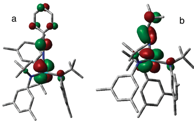
Figure 10. SOMOs of 1- [\eta^1\text{-NCPH}] (a) and 1- [\eta^1\text{-NCNMe}_2] (b) calculated at the BP86/6-311G(d,p) (MWB28 with an additional set of f functions for Mo) level.
