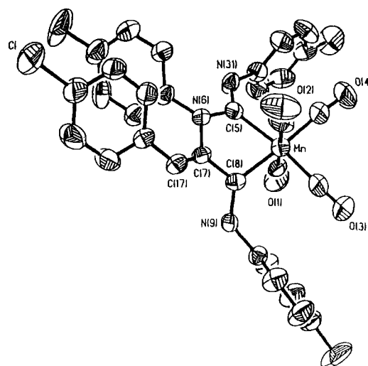
Figure 6. Molecular structure of [(\text{CO})_4\text{Mn}[\text{C}(\text{NH}-p\text{-tolyl})\text{C}\equiv\text{CH}(\text{C}_6\text{H}_4-p\text{-Cl})\text{N}(p\text{-tolyl})\text{C}(\text{NH}-p\text{-tolyl})]]^+ (6a).
