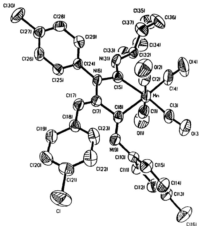
Figure 5. Molecular structure of (\text{CO})_4\text{Mn}[\text{C}(=\text{N}-p\text{-tolyl})\text{C}\equiv\text{CH}(\text{C}_6\text{H}_4-p\text{-Cl})\text{N}(p\text{-tolyl})\text{C}(\text{NHC}_6\text{H}_{11})] (4c).
