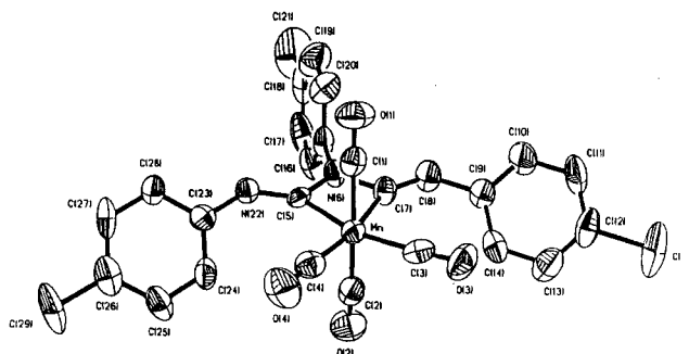
Figure 2. Molecular structure of (\text{CO})_4\text{Mn}[\text{C}\equiv\text{CH}(\text{C}_6\text{H}_4\text{-}p\text{-Cl})]\text{N}(\text{p-tolyl})\text{C}(\text{NH-}p\text{-tolyl}) ( 3a ).
