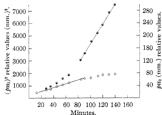
Fig. 4.—Reduction of nickel oxide containing 5 mole % chromium oxide, t = 348^\circ , p_{\text{H}_2} = 470 mm.: O, linear plot; ●, parabolic plot.
