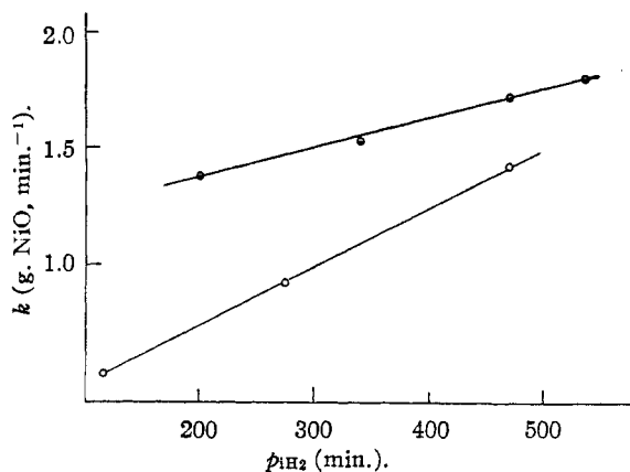
Fig. 2.—Effect of p_{\text{H}_2} on the rate of reduction of nickel oxide: \odot , t = 192^\circ ( \text{NiO} ); \circ , t = 348^\circ ( \text{NiO} + 5 mole % \text{Cr}_2\text{O}_3 ).
