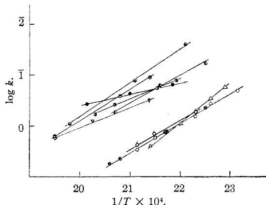
Fig. 3.—Effect of additions to nickel oxide on its rate of reduction: O, NiO fired in air or oxygen; ◊, NiO fired in helium; ⊕, NiO + 1 mole % \text{Al}_2\text{O}_3 ; ⊗, NiO + 1 mole % \text{ThO}_2 ; Δ, NiO + 1 mole % \text{Ag}_2\text{O} ; ▽, NiO + 1 mole % \text{NiCl}_2 ; ●, NiO + 1 mole % \text{MgO} ; ◐, NiO + 1 mole % \text{Cr}_2\text{O}_3 ; ◑, NiO + 1 mole % \text{Li}_2\text{O} ; ◒, NiO + 5 mole % \text{Li}_2\text{O} ; ◓, NiO + 0.5 mole % \text{WO}_3 .
