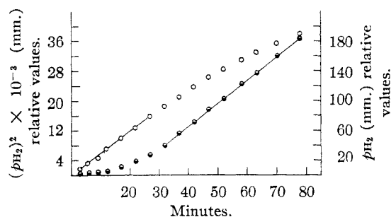
Fig. 5.—Reduction of nickel oxide containing 15 mole % chromium oxide, t = 308^\circ , p_{\text{H}_2} = 470 mm.: O, linear plot; ●, parabolic plot.
