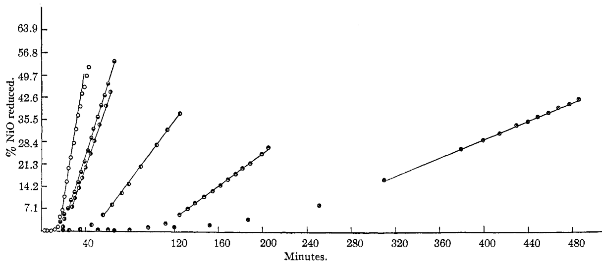
Fig. 1.—Reduction of nickel oxide by hydrogen: p_{\text{H}_2} = 470 mm.: \odot , t = 155^\circ ; \odot , t = 170^\circ ( \text{NiO} + 1.5 atom % Ni); \bullet , t = 174^\circ ; \bullet , t = 192^\circ ( \text{NiO} prepared in helium); \bullet , t = 192^\circ ( \text{NiO} prepared in oxygen); \circ , t = 200^\circ .
