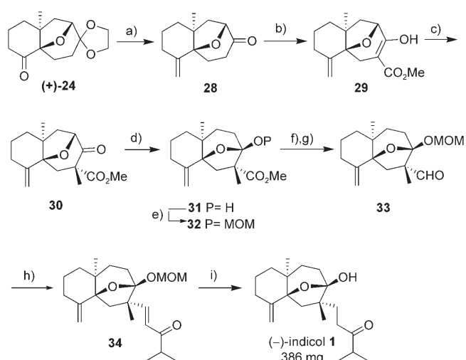
Scheme 7. a) Ph 3 PCH 3 Br, 1.6 M n BuLi, THF, 2 h, RT, then, 3 M HCl, overnight, reflux, 95 %; b) LDA, THF, 1 h, –78 °C; NCCO 2 Me, 2 h, –78 °C, 0.005 M, 88 %; c) NaH, THF, 1 h, RT; MeI, 2 h, RT, 0.005 M, 81 %; d) SmI 2 , MeOH, THF, 1 h, 0 °C, 0.002 M, 91 %; e) MOMCl, i Pr 2 NEt, CH 2 Cl 2 , 156 h, RT, 92 %; f) LAH, Et 2 O, 4 h, RT; g) DMSO, (COCl) 2 , CH 2 Cl 2 ; Et 3 N, 10 min, –78 °C; h) NaH, dimethyl(3-methyl-2-oxobutyl)-phosphonate, THF, overnight, RT, 90 % over 3 steps from 36 ; i) [Ph 3 P(CuH)] 6 , THF, H 2 O, 24 h, RT; then 12 M HCl, MeOH, 48 h, RT, 98 %. MOM = methoxymethyl.
