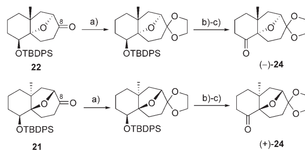
Scheme 4. For 22 : a) \text{TMSCH}_2\text{CH}_2\text{OTMS} , \text{TMSOTf} , \text{CH}_2\text{Cl}_2 , overnight, RT, 93%; b) 1 M \text{TBAF} , THF, 40 h, reflux; c) \text{DMSO} , (\text{COCl})_2 , \text{CH}_2\text{Cl}_2 ; \text{NEt}_3 , 10 min, -78^\circ\text{C} , 82% for 2 steps. For 21 : a) \text{TMSOCH}_2\text{CH}_2\text{OTMS} , \text{TMSOTf} , \text{CH}_2\text{Cl}_2 , overnight, RT; b) 1 M \text{TBAF} , 64 h, RT, 99% over 2 steps; c) \text{DMSO} , (\text{COCl})_2 , \text{CH}_2\text{Cl}_2 ; \text{NEt}_3 , 10 min, -78^\circ\text{C} , 98%. \text{TMS} = trimethylsilyl; \text{OTf} = triflate; \text{TBAF} = tetrabutylammonium fluoride.
