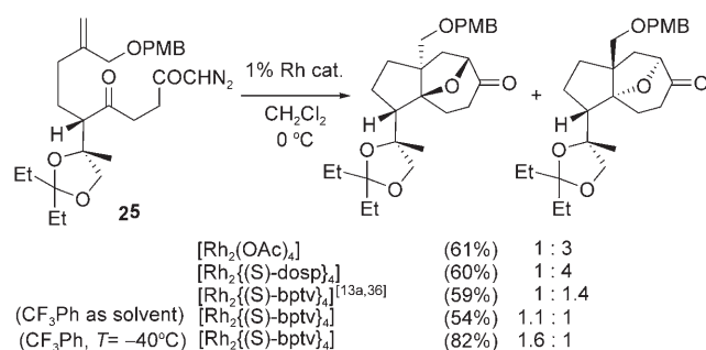
Scheme 6. CCCC reaction of 25 containing a three-carbon tether.
