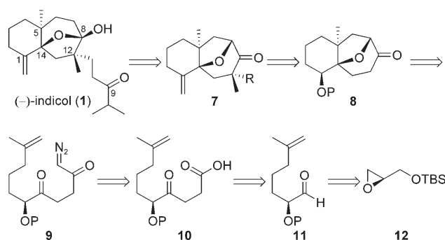
Scheme 1. Retrosynthetic analysis of indicol.
