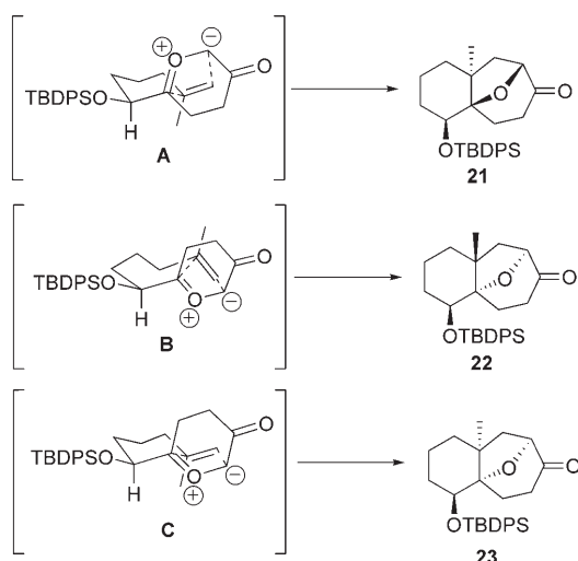
Scheme 5. Proposed transition states of the cycloaddition of the carbonyl ylide.
