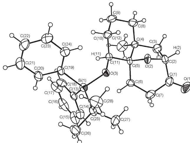
Figure 1. ORTEP of cycloadduct (±)- 21 .
