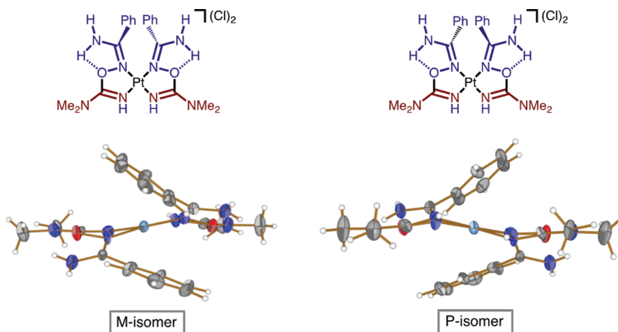
Figure 4. Isomerism for [8b](Cl)_2 .
