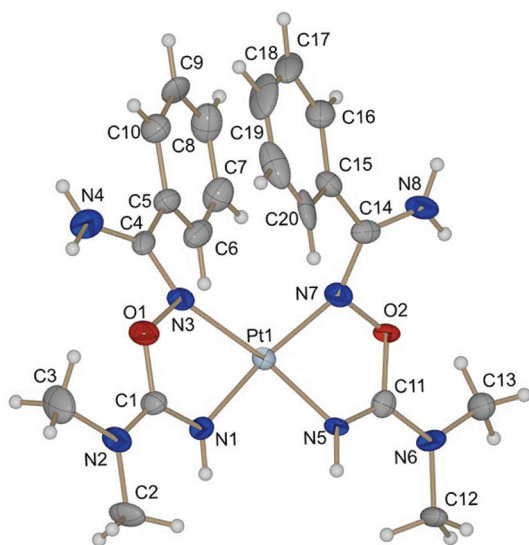
Figure 3. Molecular structure of P\text{-}[\mathbf{8b}](\text{Cl})_2 with the atomic numbering scheme. Cl anions are omitted for clarity. Thermal ellipsoids are given at the 50% probability level. Selected bond lengths (Å): N1–C1 1.316(10); N5–C11 1.299(10); N2–C1 1.314(11); N6–C11 1.339(10); N3–C4 1.320(10); N7–C14 1.316(11); N4–C4 1.321(11); N8–C14 1.308(11).
