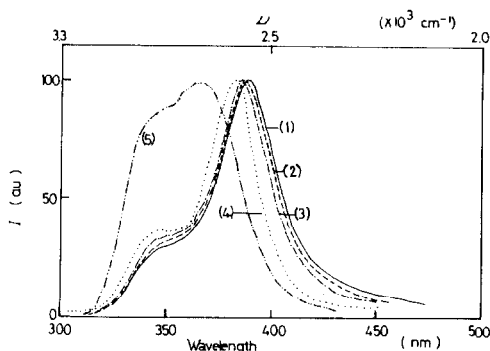
Fig. 4. The dependence of emission spectra on \text{Ce}^{3+} ion content in \text{Ce}^{3+} -film system. (1) 0.11%; (2) 0.22%; (3) 0.33%; (4) 1.10%; (5) 3.0%.
