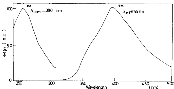
Fig. 3. The excitation and fluorescence spectra of PMMA film alone.
