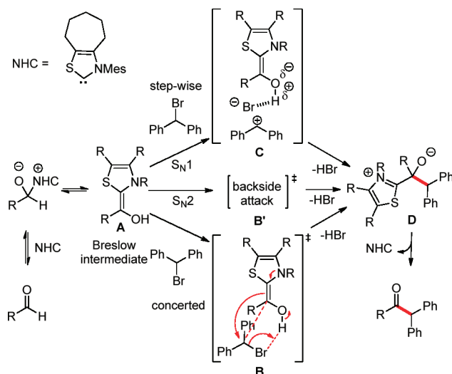
Scheme 5. Possible Mechanistic Pathways
