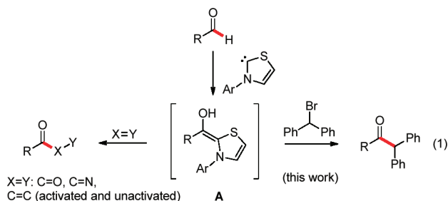
Scheme 1. NHC-Catalyzed Umpolung of Aldehydes
