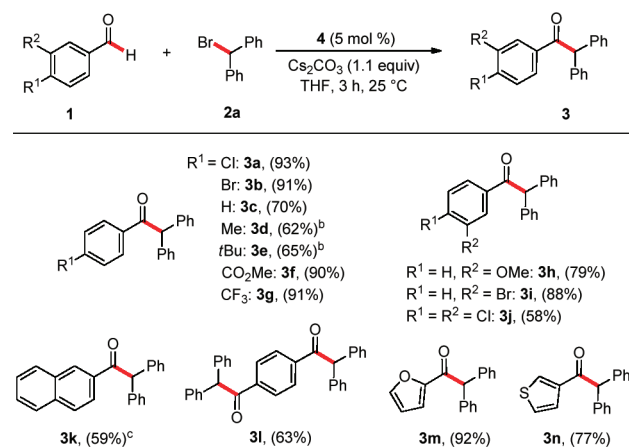
Scheme 2. NHC-Catalyzed Alkylation of Aldehydes: Variation of the Aldehyde Moiety a
