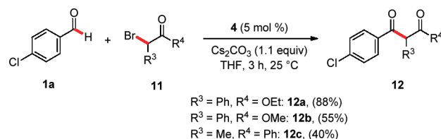
Scheme 6. Utility of α-Bromo Esters and α-Bromo Ketone
