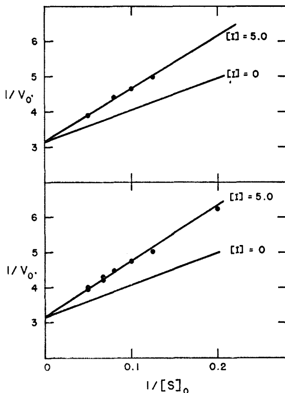
Fig. 2.—Both curves, substrate, nicotinyl-L-tryptophanamide; [E] 0.208 mg. of protein-nitrogen per ml.; [S], [I] in units of 10^{-3} M; upper curve, inhibitor, nicotinyl-D-phenylalaninamide; lower curve, inhibitor, nicotinyl-D-tyrosinamide.
