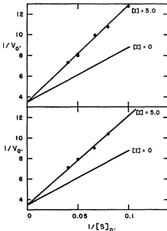
Fig. 4.—Both curves, substrate, nicotinyl-L-tyrosinamide; [E] 0.047 mg. of protein-nitrogen per ml.; [S], [I] in units of 10^{-3} M; upper curve, inhibitor, nicotinyl-D-tyrosinamide; lower curve, inhibitor, nicotinyl-D-phenylalaninamide.
