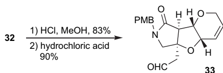
Scheme 10. Further chemoselective transformation on the cis -fused heterotricycle 32 .
