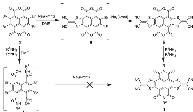
Scheme 2. Proposed Reaction Process of the One-Pot Synthesis
