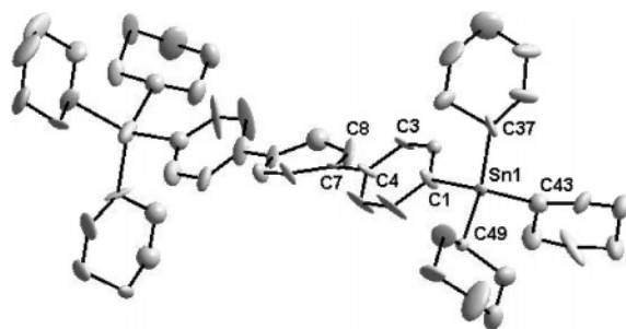
Figure 1. Molecular structure of 2. Thermal ellipsoids are shown at the 50% probability level. Hydrogen atoms are omitted for clarity. Selected distances (Å) and angles (deg): Sn1–C1 2.147(12), Sn1–C43 2.161(13), Sn1–C49 2.166(9), Sn1–C37 2.169(14), C1–Sn1–C43 101.6(5), C1–Sn1–C49 109.3(4), C43–Sn1–C49 112.7(5), C1–Sn1–C37 107.5(6), C43–Sn1–C37 109.1(5), C49–Sn1–C37 115.6(5), C3–C4–C7–C8 30.1(1).
