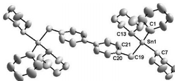
Figure 2. Molecular structure of 3. Thermal ellipsoids are shown at the 50% probability level. Hydrogen atoms are omitted for clarity. Selected distances (Å) and angles (deg): Sn1–C1 2.147(12), Sn1–C7 2.182(7), Sn1–C19 2.156(9), Sn1–C13 2.180(9), C1–Sn1–C19 110.2(5), C1–Sn1–C13 115.1(4), C13–Sn1–C19 110.5(4), C1–Sn1–C7 109.0(4), C7–Sn1–C19 103.3(3), C7–Sn1–C13 108.1(3), Sn1–C19–C20 117.5(6), Sn1–C19–C20–C21 77.0(1).
