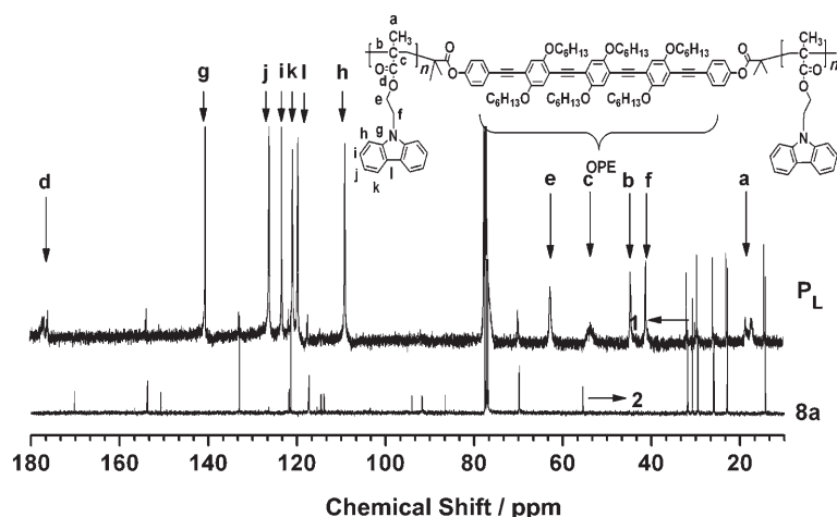
Figure 3. ^{13}\text{C} NMR spectra of 8a and the related block copolymer ( P L ) in \text{CDCl}_3 .
