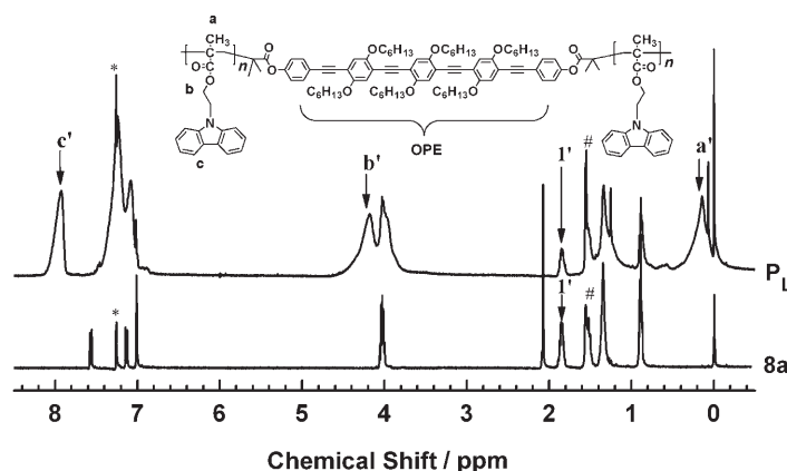
Figure 2. 1 H NMR spectra of 8a and the related block copolymer ( P L ) in CDCl 3 . (Symbols * and # represent peaks from CDCl 3 and H 2 O, respectively).
