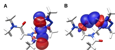
Figure 4. Orbital overlaps stabilizing the preferred conformation of II : (A) n \rightarrow \pi^*_{\text{Ar}} delocalization; (B) H-bonding interaction ( n \rightarrow \sigma^* ).
