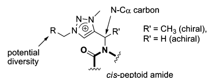
Figure 2. Structure of cis -directing triazolium-type peptoid side chains.
